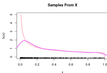
Figure 6.3: Learning a distribution using kernel density estimation.
