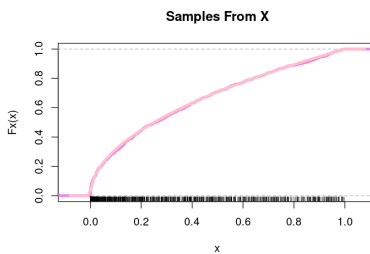
Figure 6.1: Learning a distribution using the empirical cumulative distribution function.
