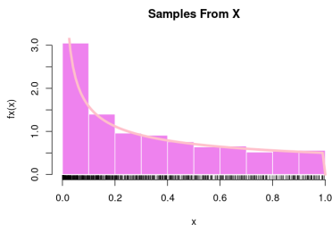
Figure 6.2: Learning a distribution using a histogram.
